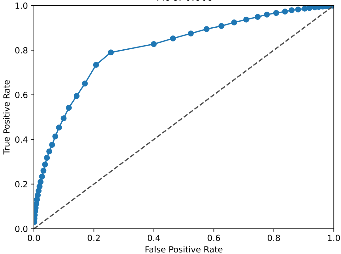
SIX4 ROC Curve AUC: 0.809
