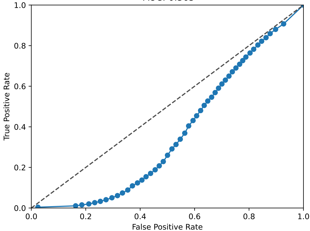
TBX15 ROC Curve AUC: 0.365
