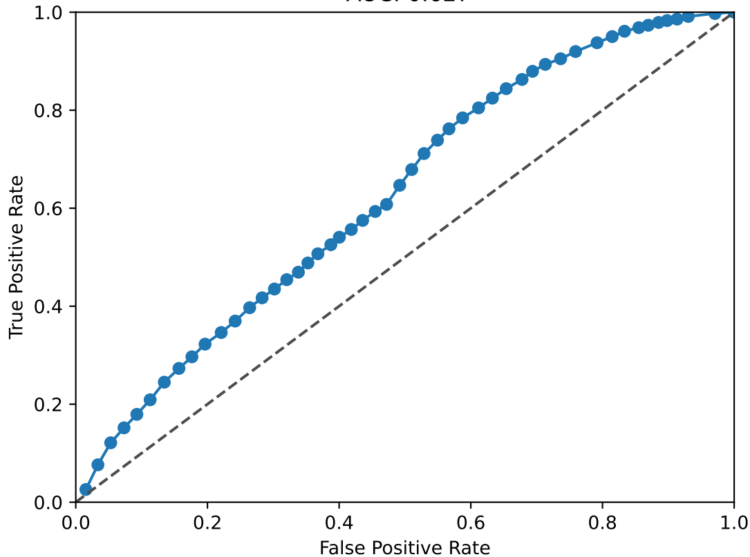
CUX2 ROC Curve AUC: 0.627
