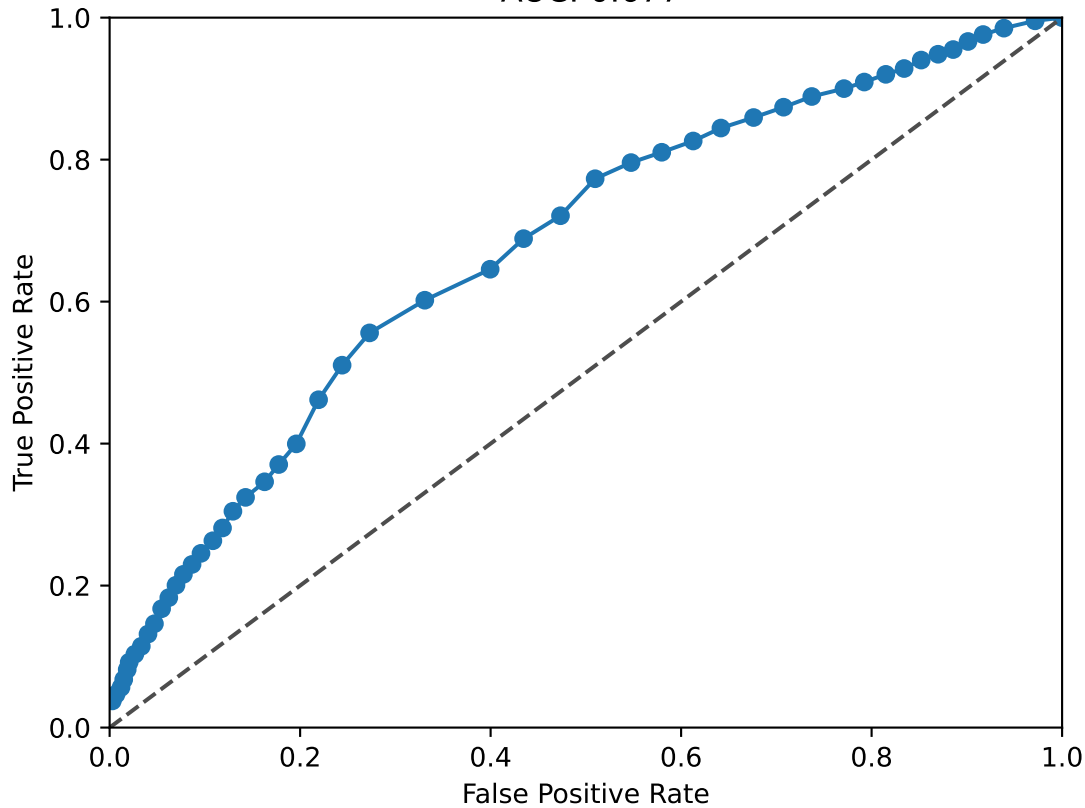
JUN ROC Curve AUC: 0.677
