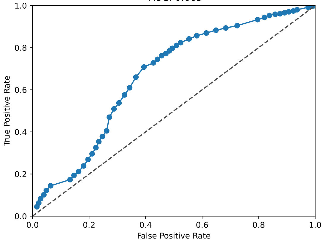
LMX1B ROC Curve AUC: 0.665
