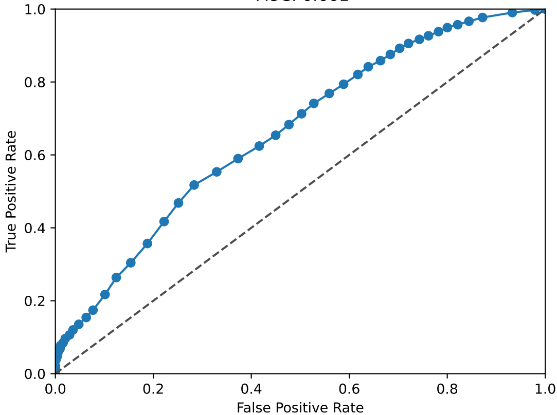
NFIA ROC Curve AUC: 0.661
