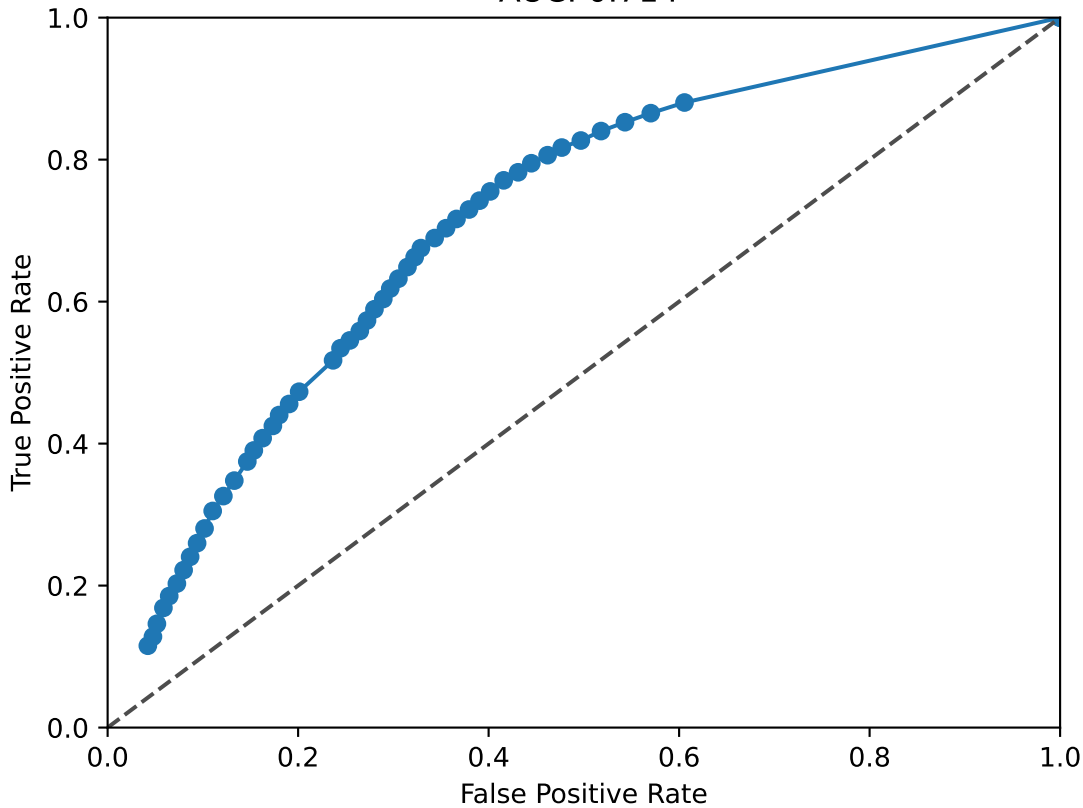
REST ROC Curve AUC: 0.714
