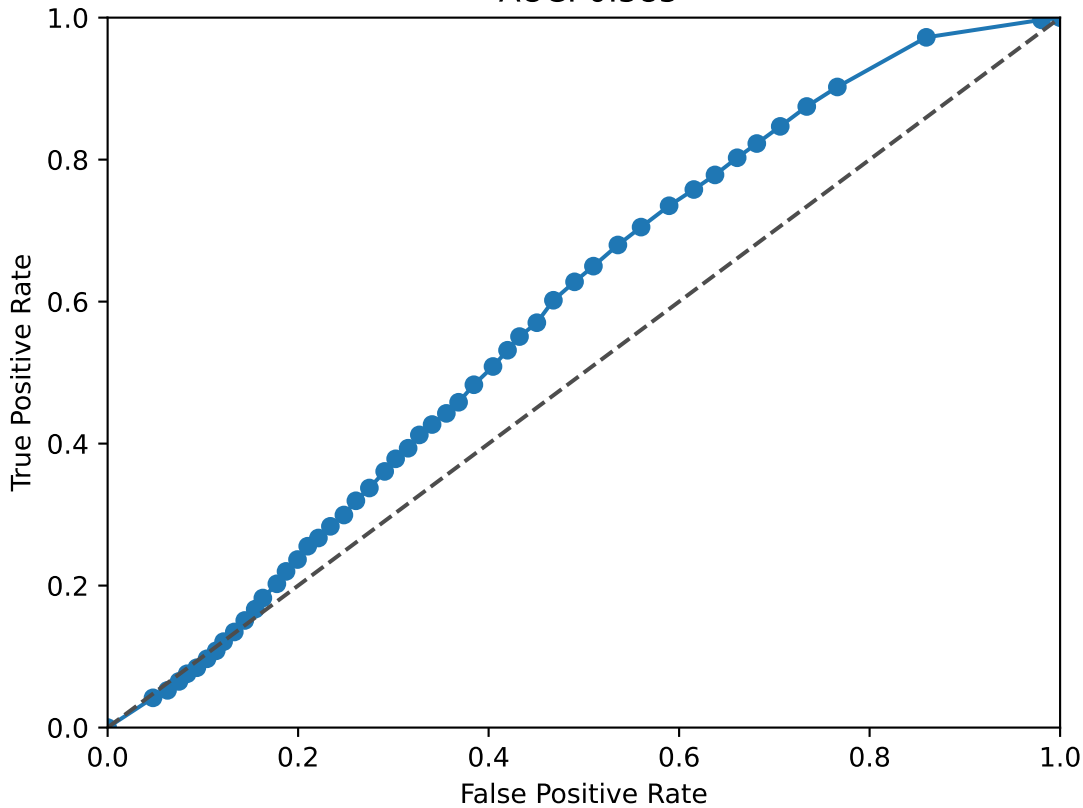
SIX1 ROC Curve AUC: 0.585
