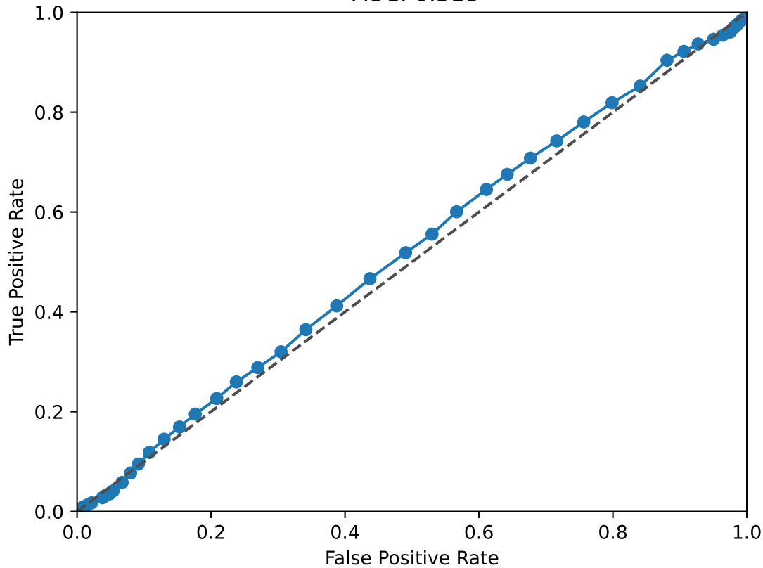
STAT2 ROC Curve AUC: 0.518
