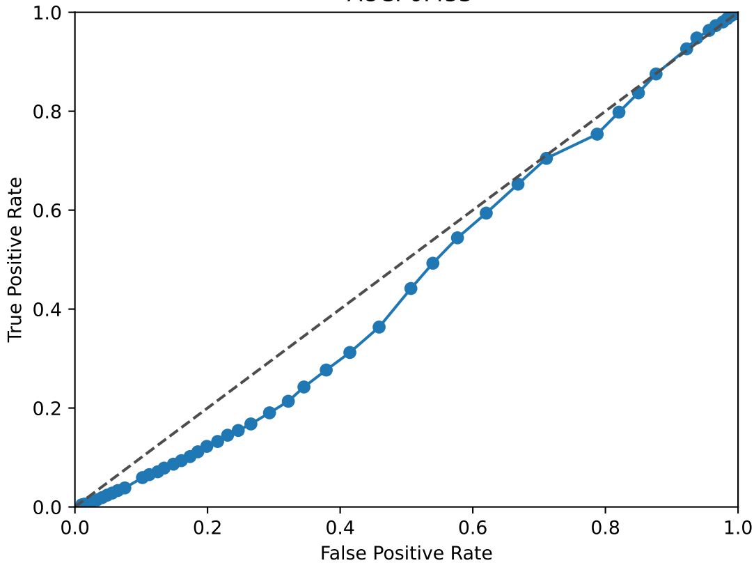
TCF7L1 ROC Curve AUC: 0.453
