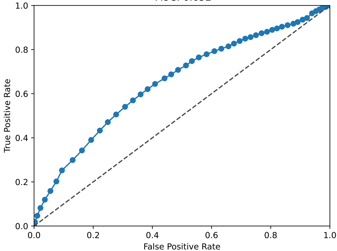
CUX2 ROC Curve AUC: 0.652
