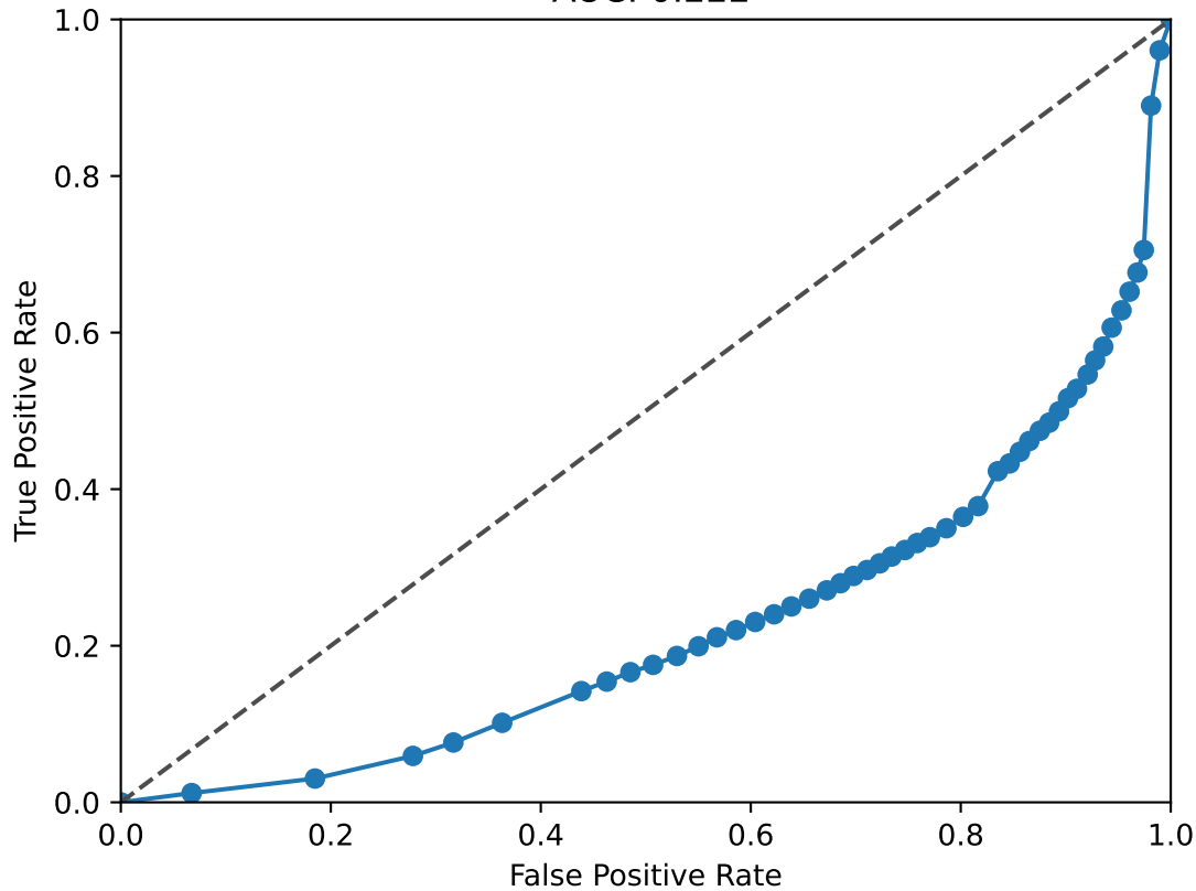
GRHL2 ROC Curve AUC: 0.222
