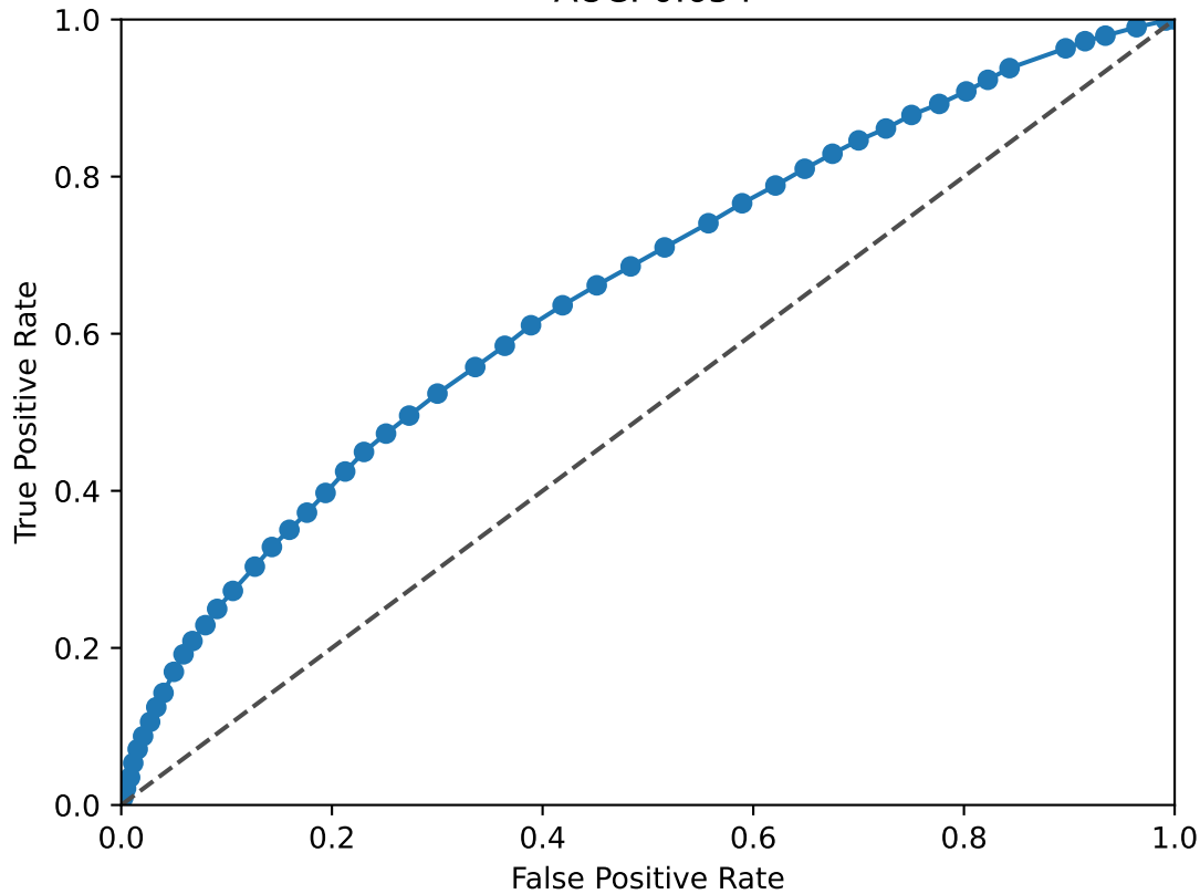
HSF2 ROC Curve AUC: 0.654
