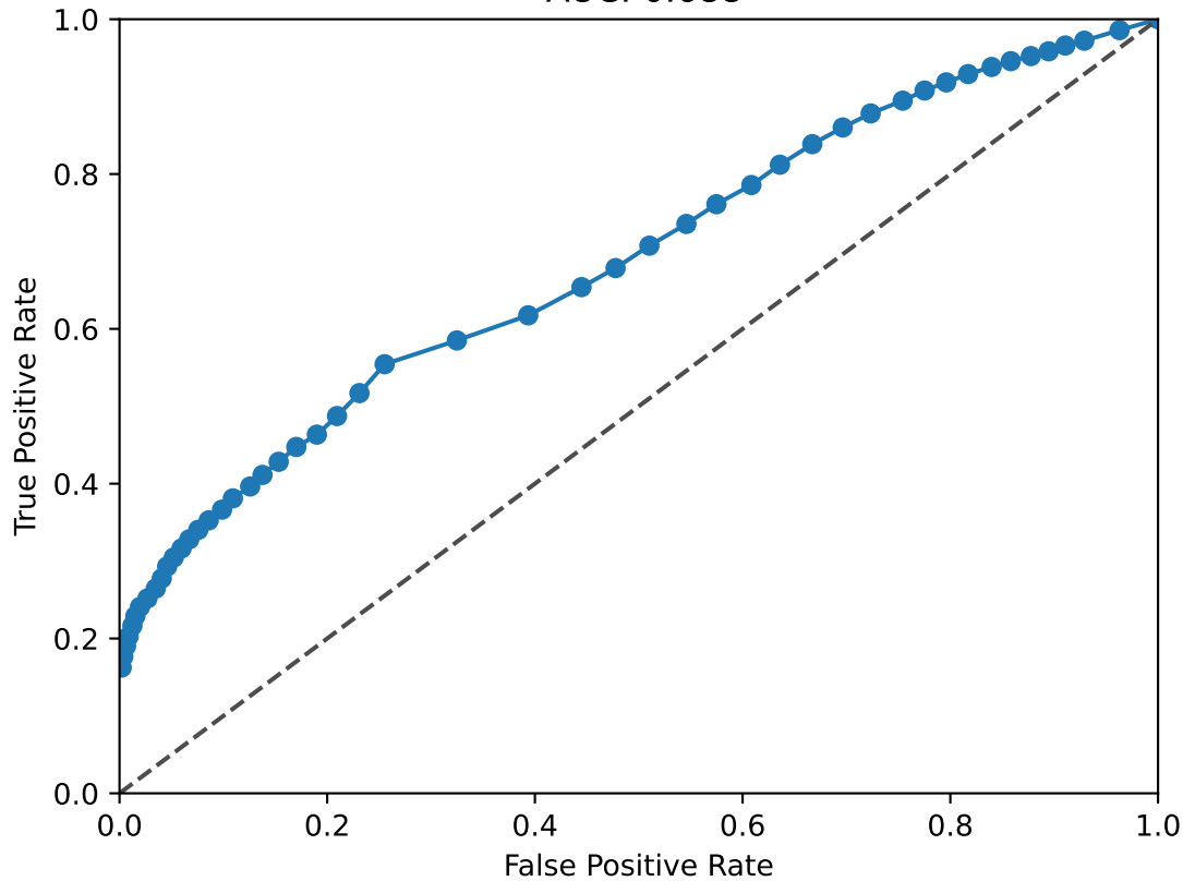
JUN ROC Curve AUC: 0.688
