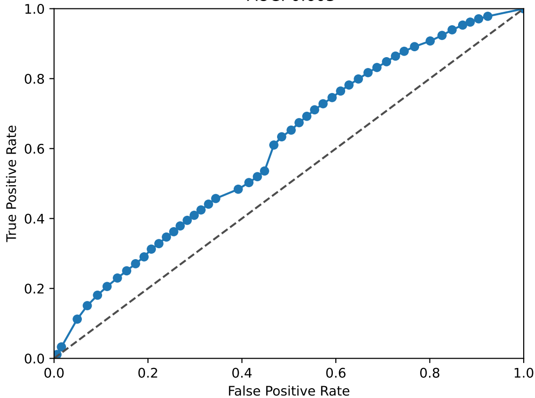
PKNOX2 ROC Curve AUC: 0.603
