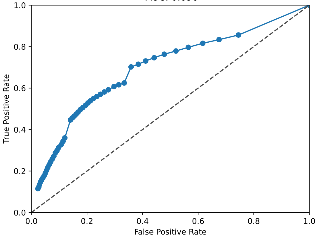
REST ROC Curve AUC: 0.696
