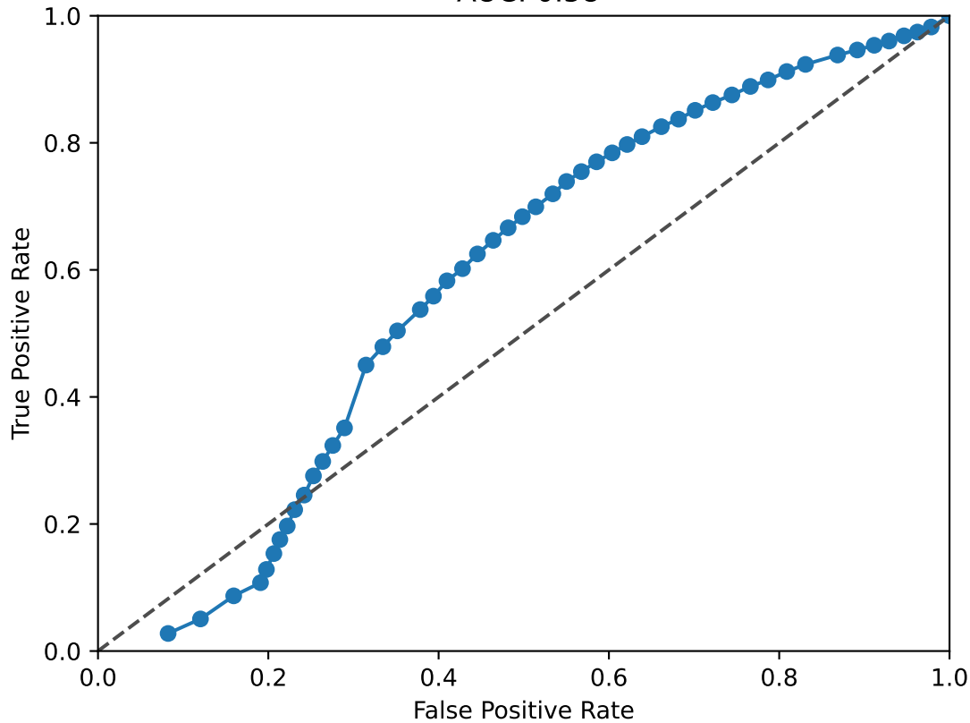
RORA_RORB ROC Curve AUC: 0.58
