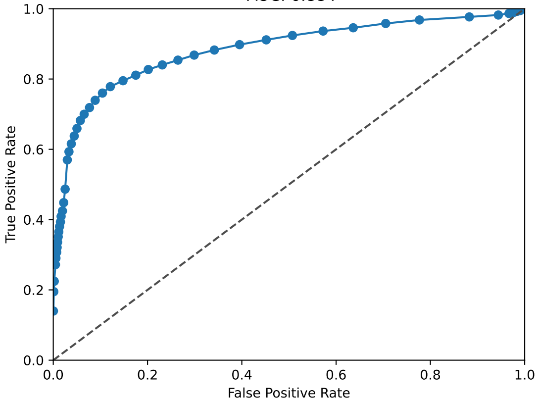
RUNX1 ROC Curve AUC: 0.884
