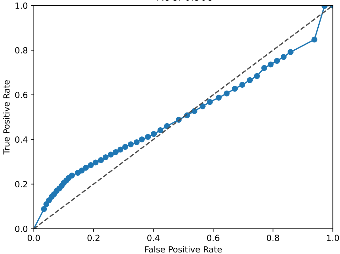
SIX1 ROC Curve AUC: 0.508
