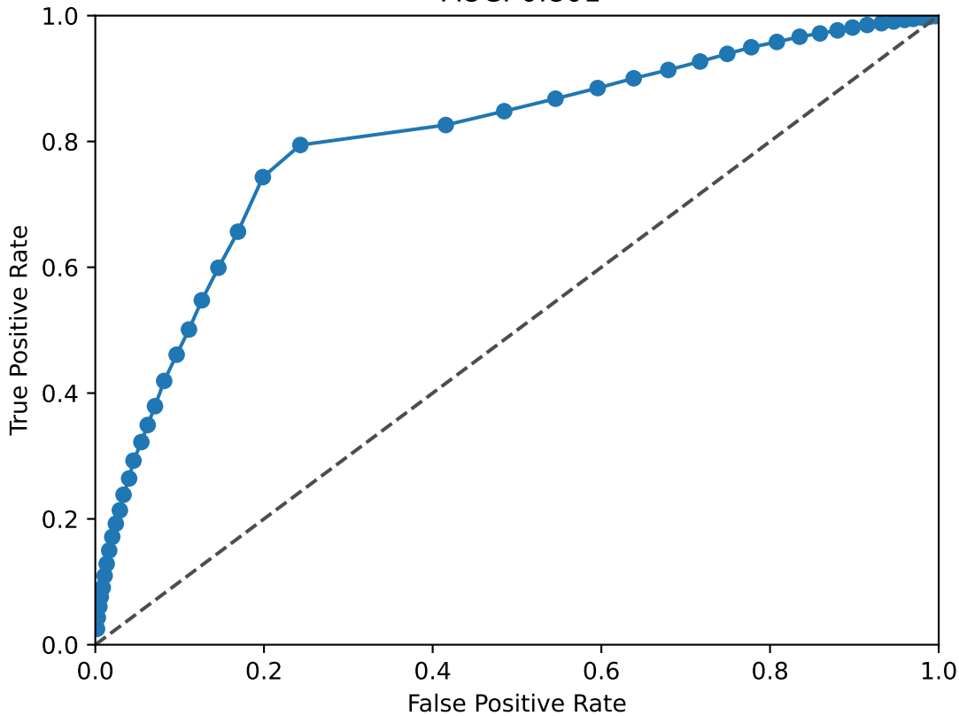
SIX4 ROC Curve AUC: 0.801
