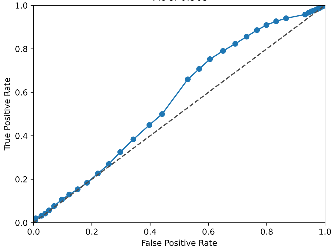
STAT2 ROC Curve AUC: 0.563
