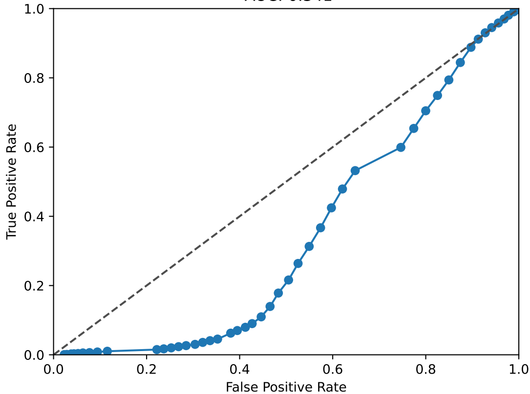
TCF7L1 ROC Curve AUC: 0.341
