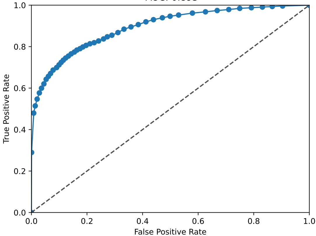
BACH1 ROC Curve AUC: 0.893
