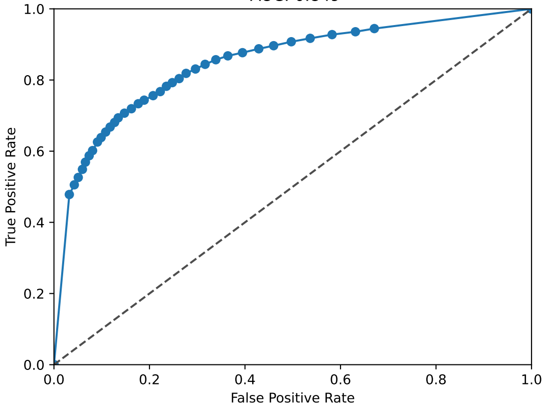
EHF ROC Curve AUC: 0.849
