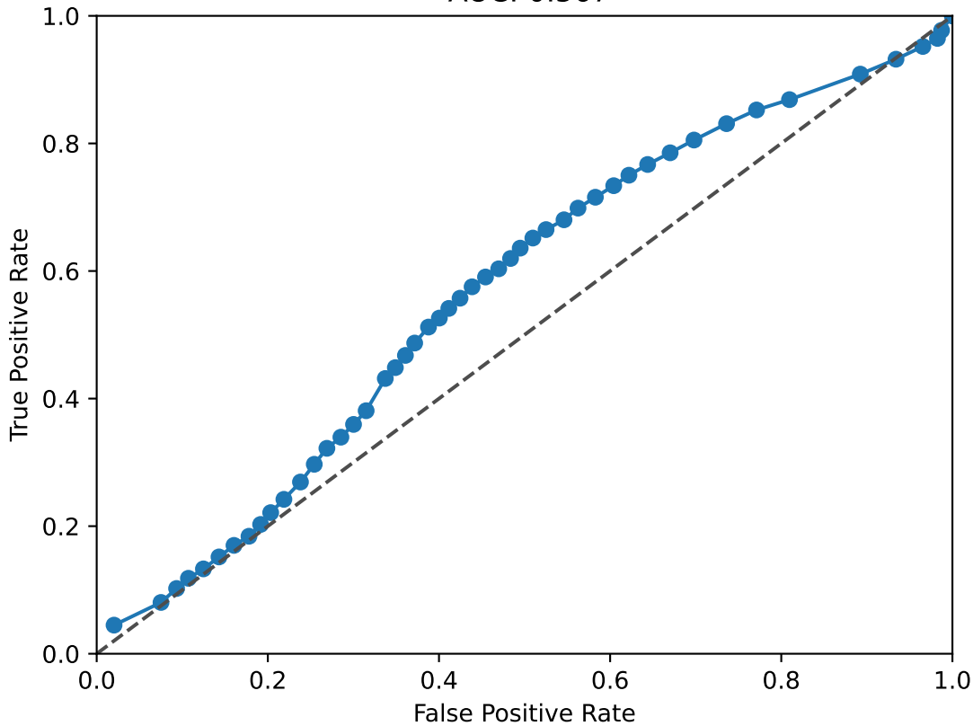
EPCAM ROC Curve AUC: 0.567
