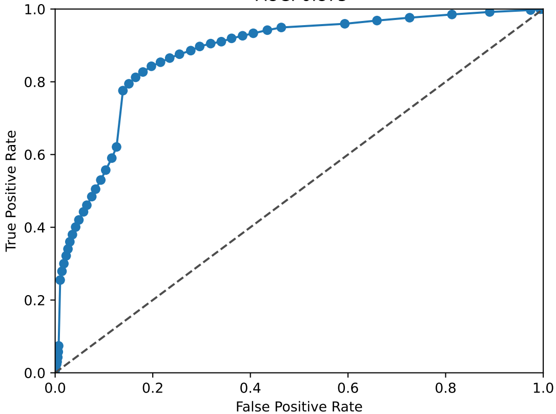
ETS1 ROC Curve AUC: 0.875
