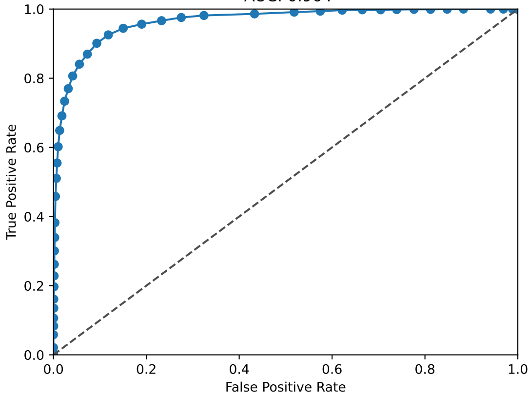
FOS ROC Curve AUC: 0.964
