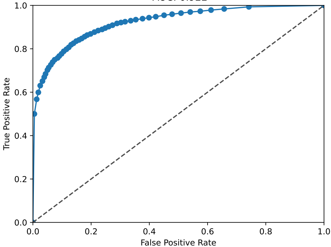
GRHL2 ROC Curve AUC: 0.922
