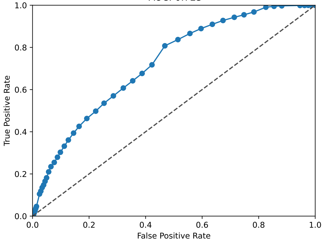
HSF2 ROC Curve AUC: 0.723
