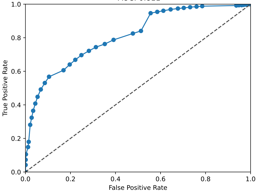
JUNB ROC Curve AUC: 0.811
