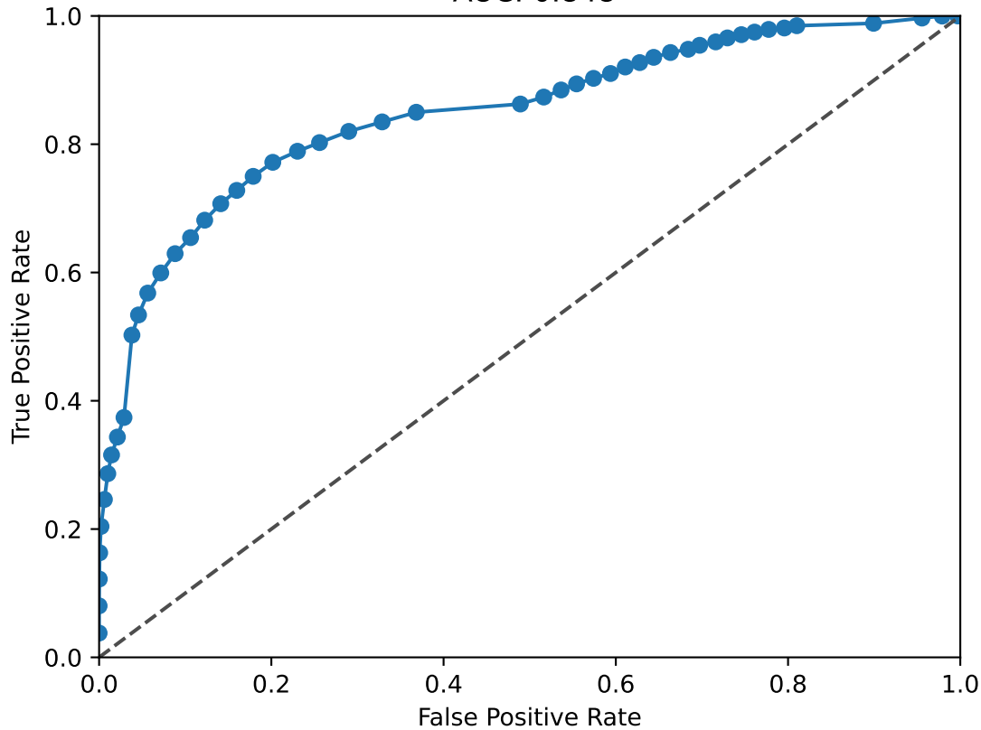
JUN ROC Curve AUC: 0.848
