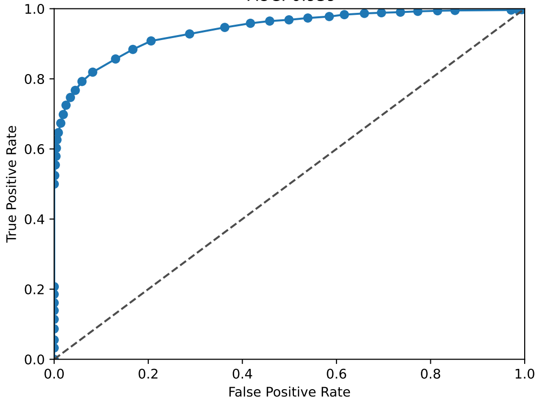
PBX1 ROC Curve AUC: 0.939
