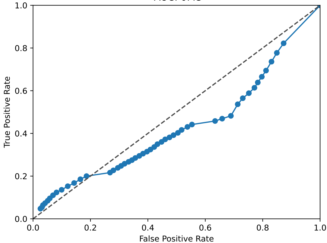
REST ROC Curve AUC: 0.43
