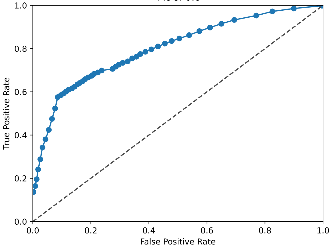
RORA_RORB ROC Curve AUC: 0.8
