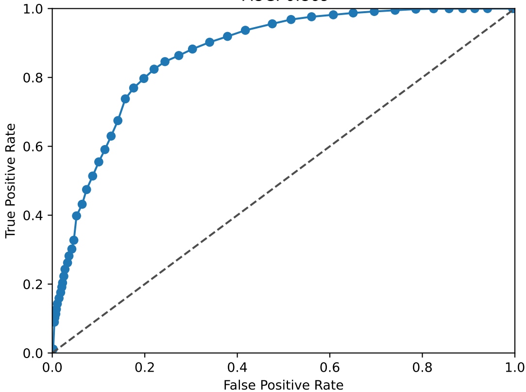
RUNX1 ROC Curve AUC: 0.869
