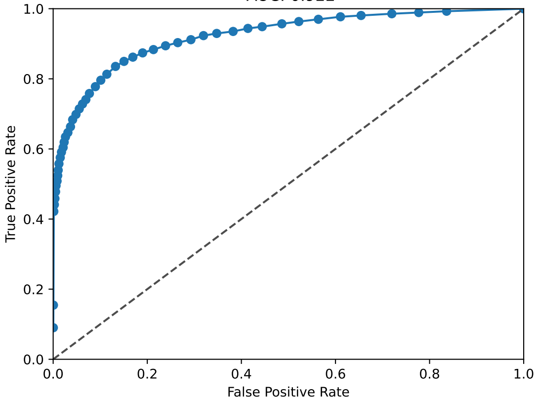
TCF7L1 ROC Curve AUC: 0.922
