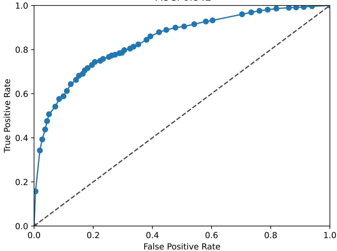
BACH1 ROC Curve AUC: 0.842
