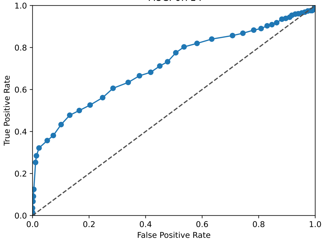
EGR1 ROC Curve AUC: 0.714
