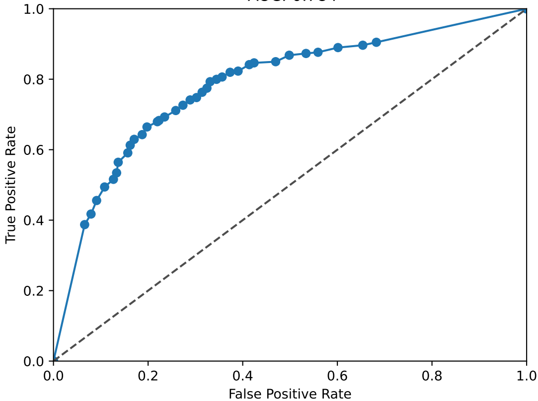
EHF ROC Curve AUC: 0.784
