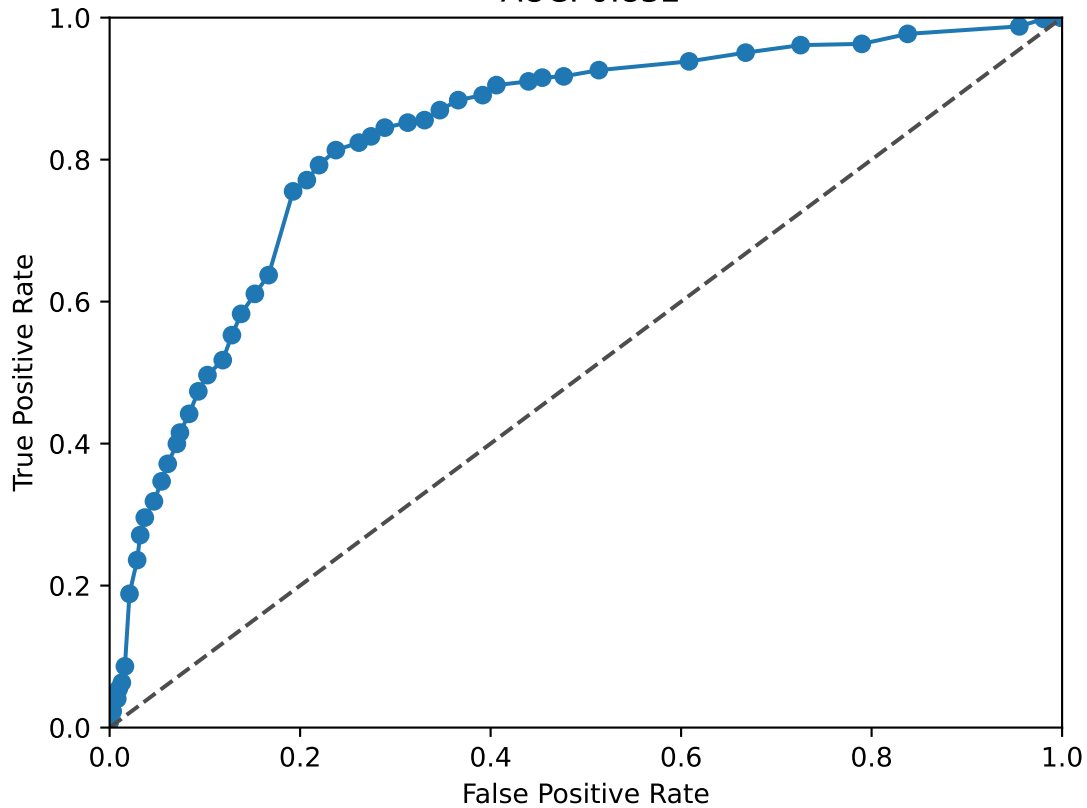
ETS1 ROC Curve AUC: 0.832
