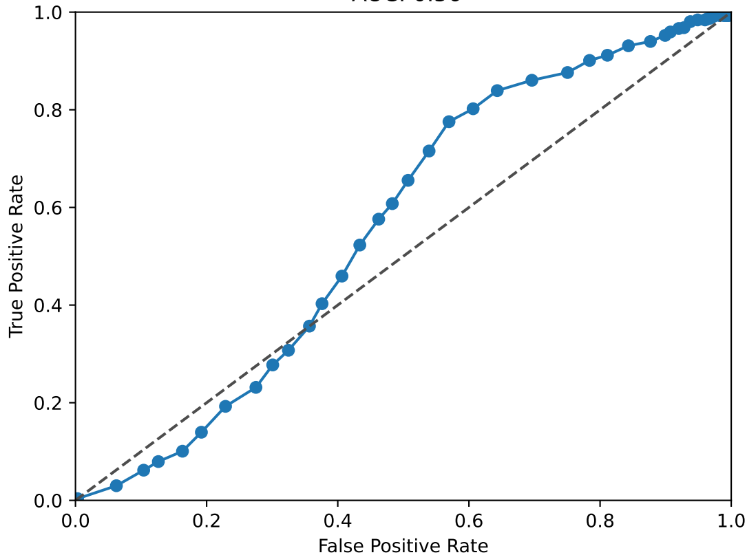
KMT2A ROC Curve AUC: 0.56
