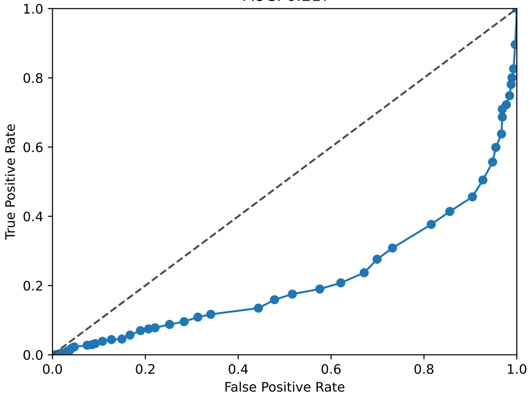
NFIX ROC Curve AUC: 0.217
