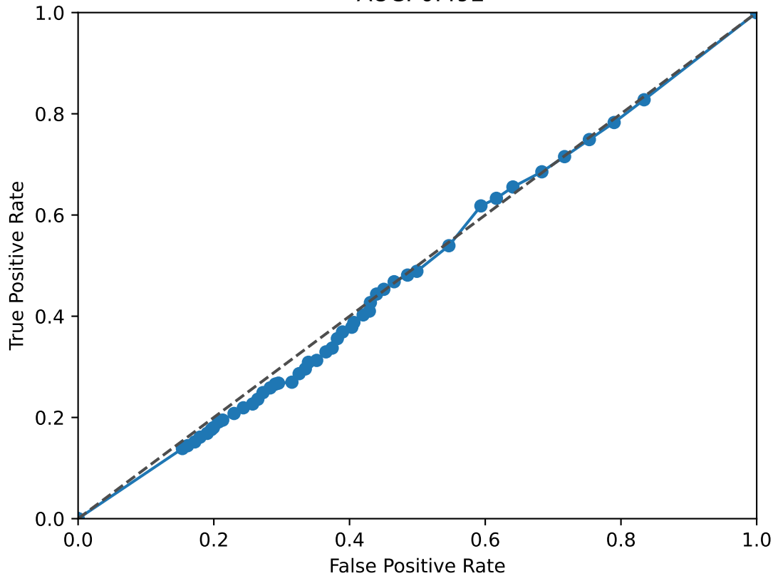
PROX1 ROC Curve AUC: 0.492
