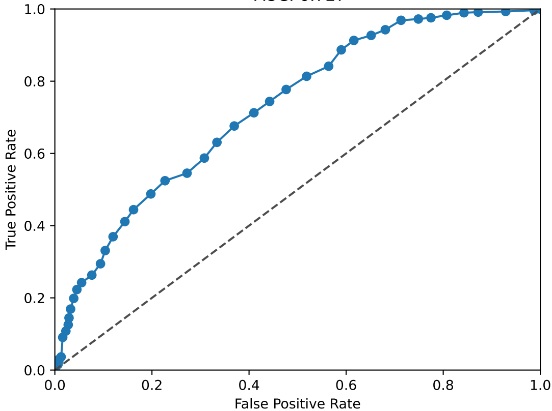
SIX4 ROC Curve AUC: 0.727
