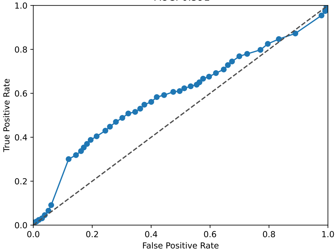
TBX15 ROC Curve AUC: 0.591
