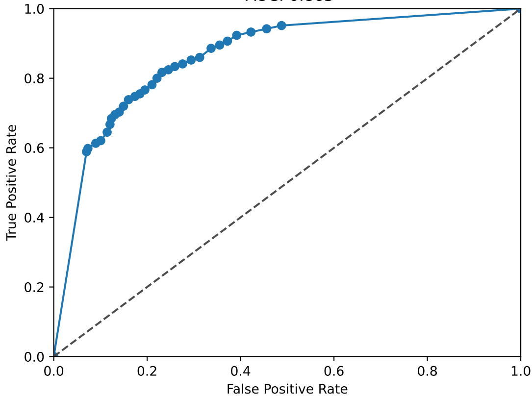
THR B ROC Curve AUC: 0.863
