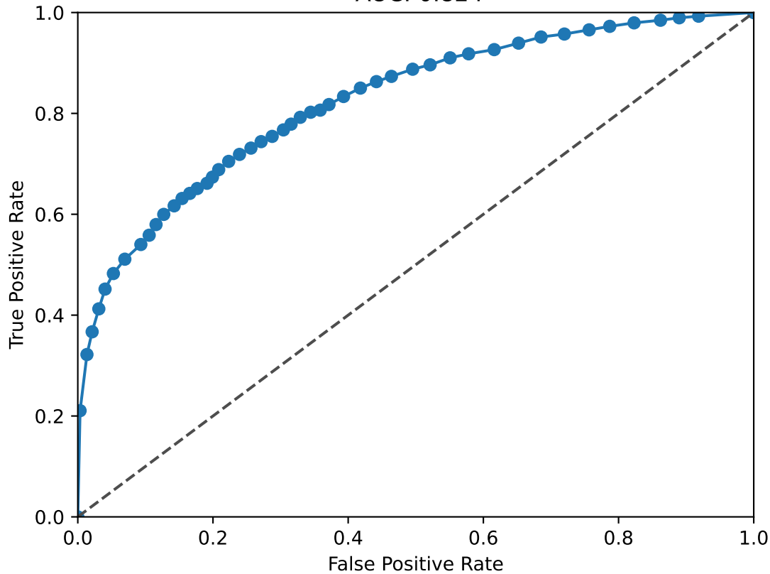
BACH1 ROC Curve AUC: 0.824
