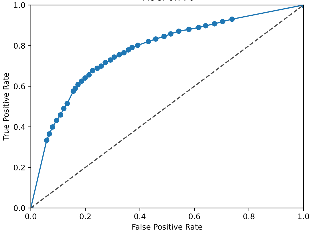
EHF ROC Curve AUC: 0.776
