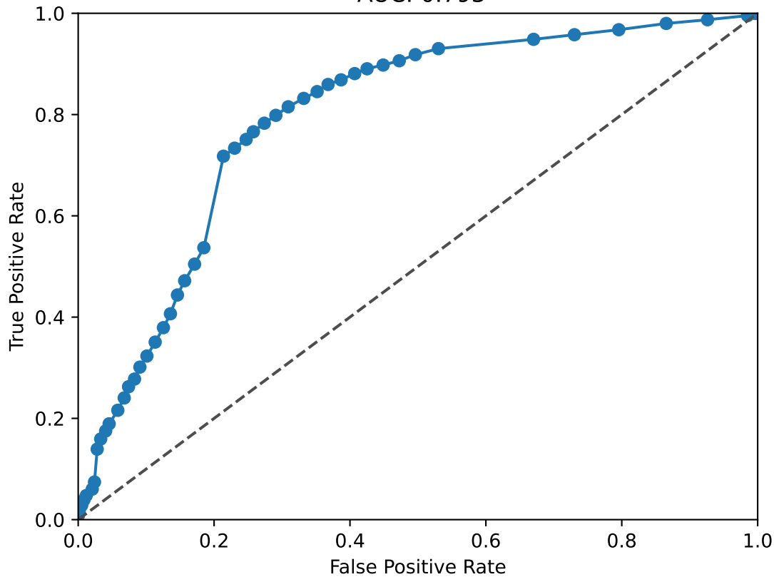
ETS1 ROC Curve AUC: 0.793
