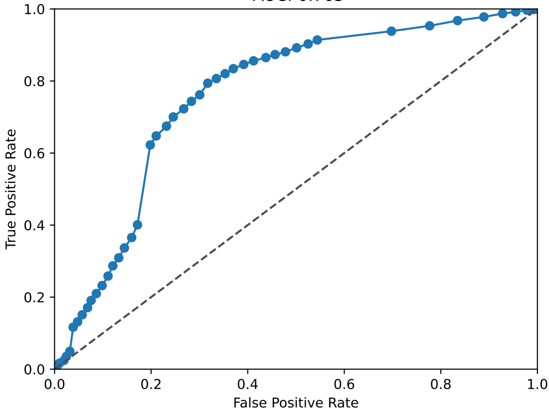
FOXO3 ROC Curve AUC: 0.763
